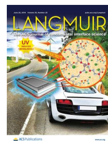
Langmuir 35 (2019) 8210-8219
