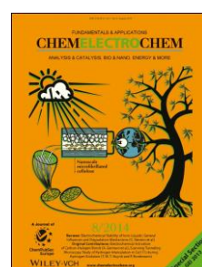
ChemElectroChem 1 (2014) 1350-1358
